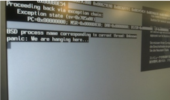
Fig. 10.4.1: A kernel panic on a BSD system. The panic message is displayed on the screen. The panic message is: "panic: We are hanging here...". The panic message is displayed on the screen. The panic message is: "panic: We are hanging here...".
